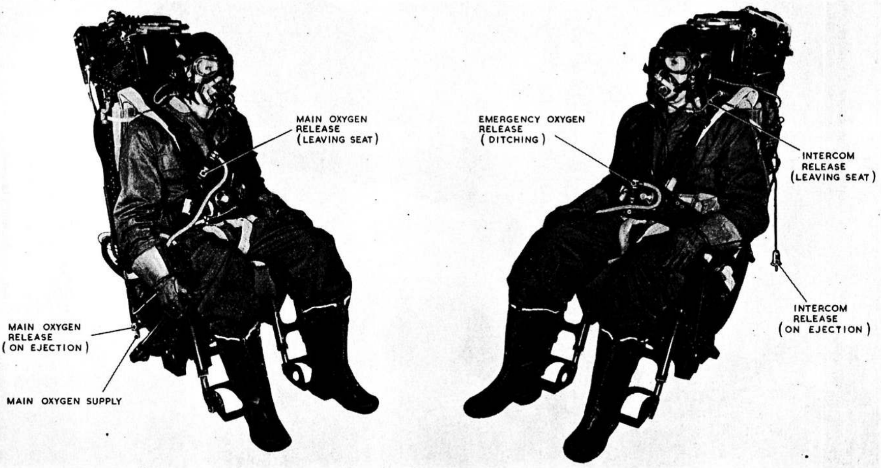
Fig. 2. Mk. 2B ejection seat (quick-release connections)
