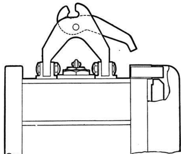
Fig. 4. Action of scissor shackle
