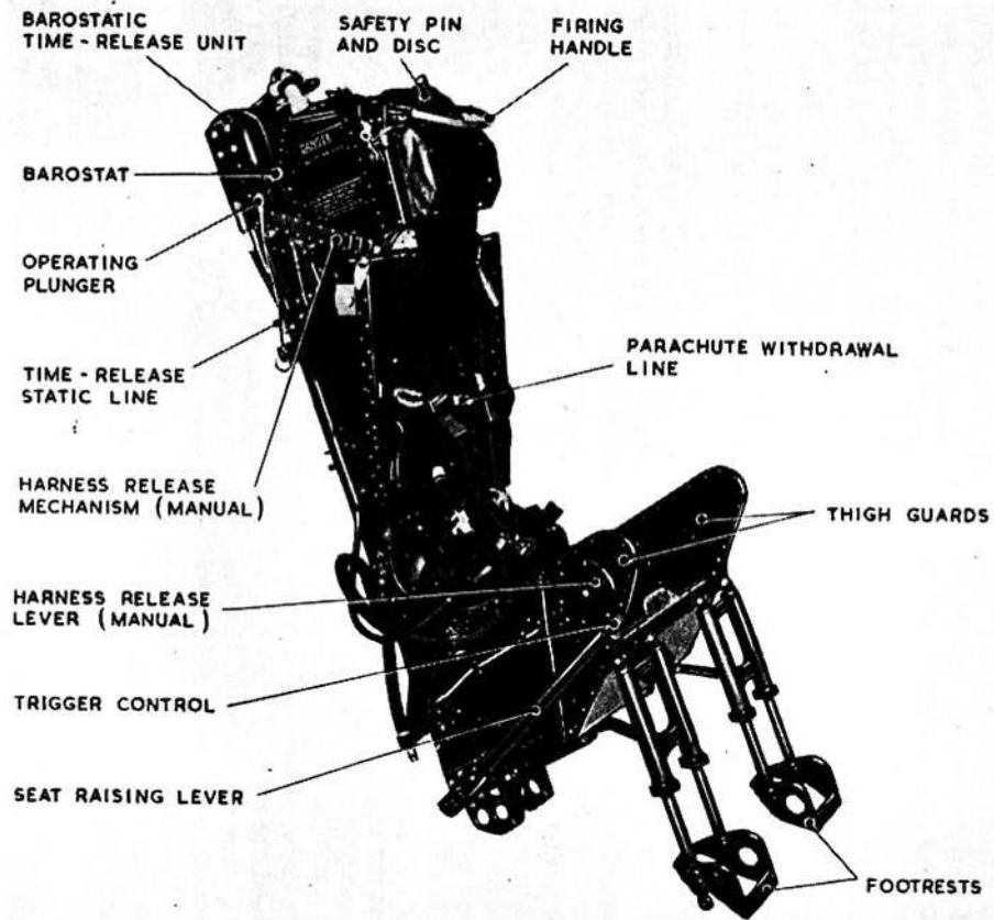
Fig. 1. Mk. 2B ejection seat (structure)
