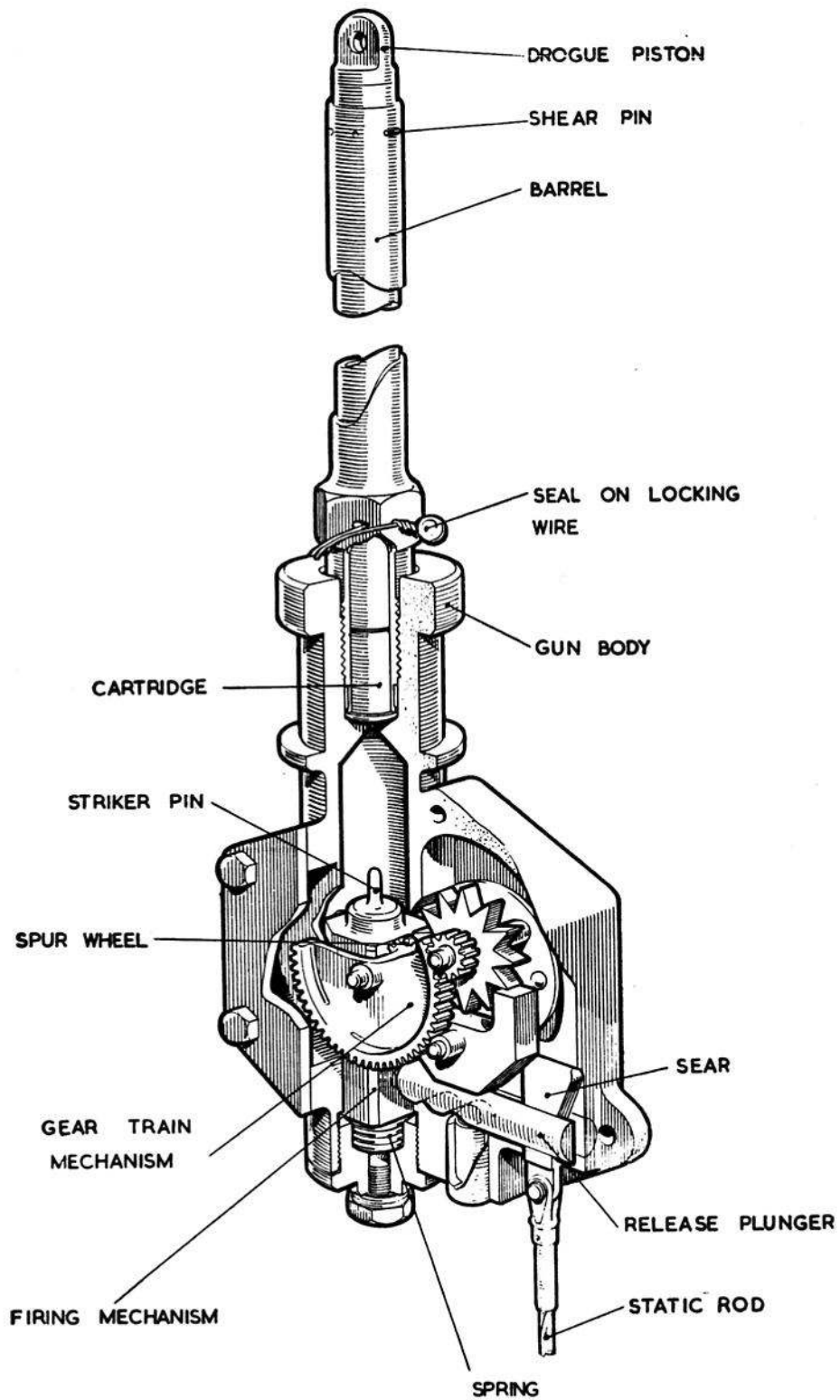
Fig. 2. Type 2 drogue gun assembly
