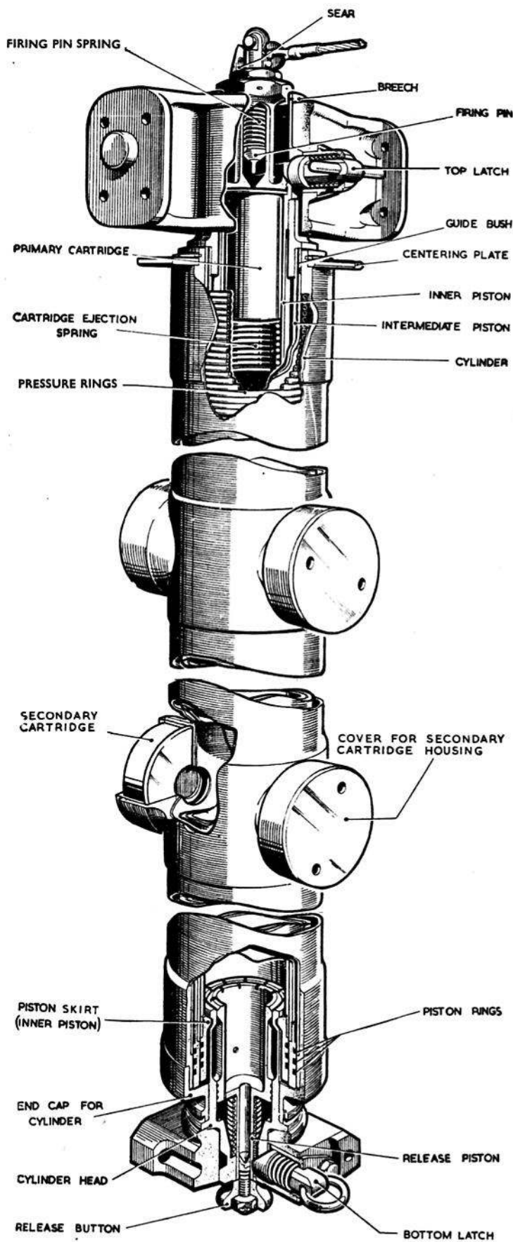
Fig. 1. Type 3 ejection gun assembly
