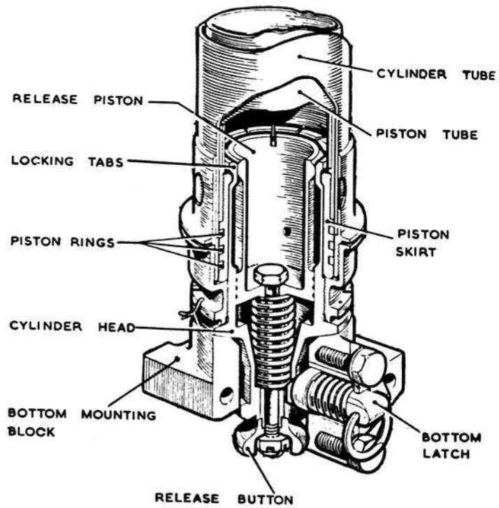
Fig. 1. Ejection gun assembly
