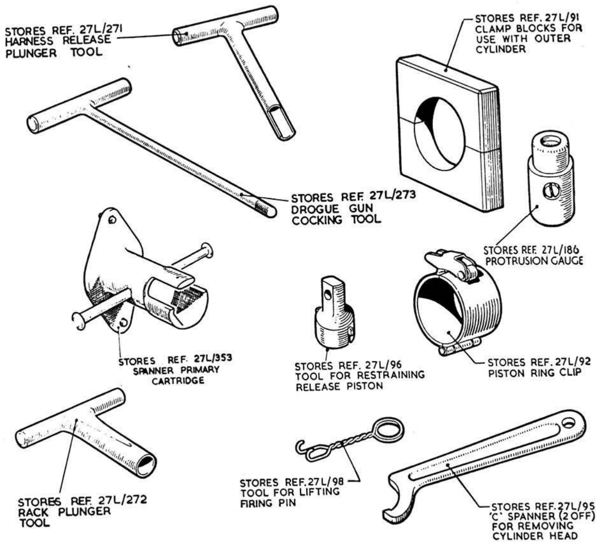
Fig. 2. Special tools (Type 1, 1A and 2 guns)
