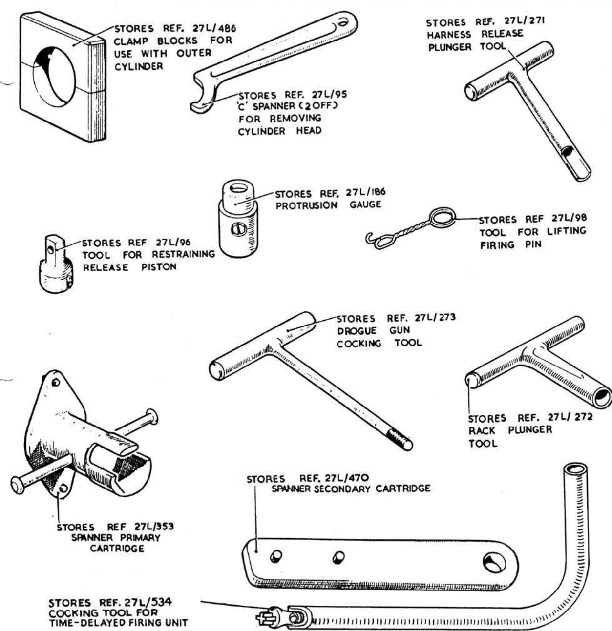
Fig. 3. Special tools (Type 3 and 3A guns)
