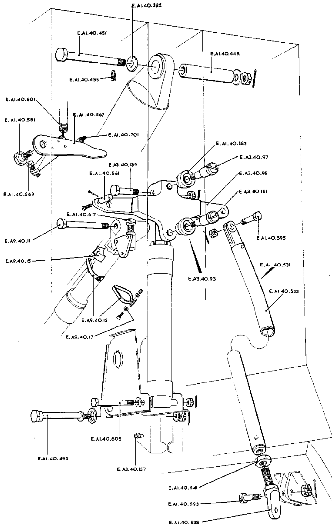
NOSEWHEEL DOOR MECHANISM
