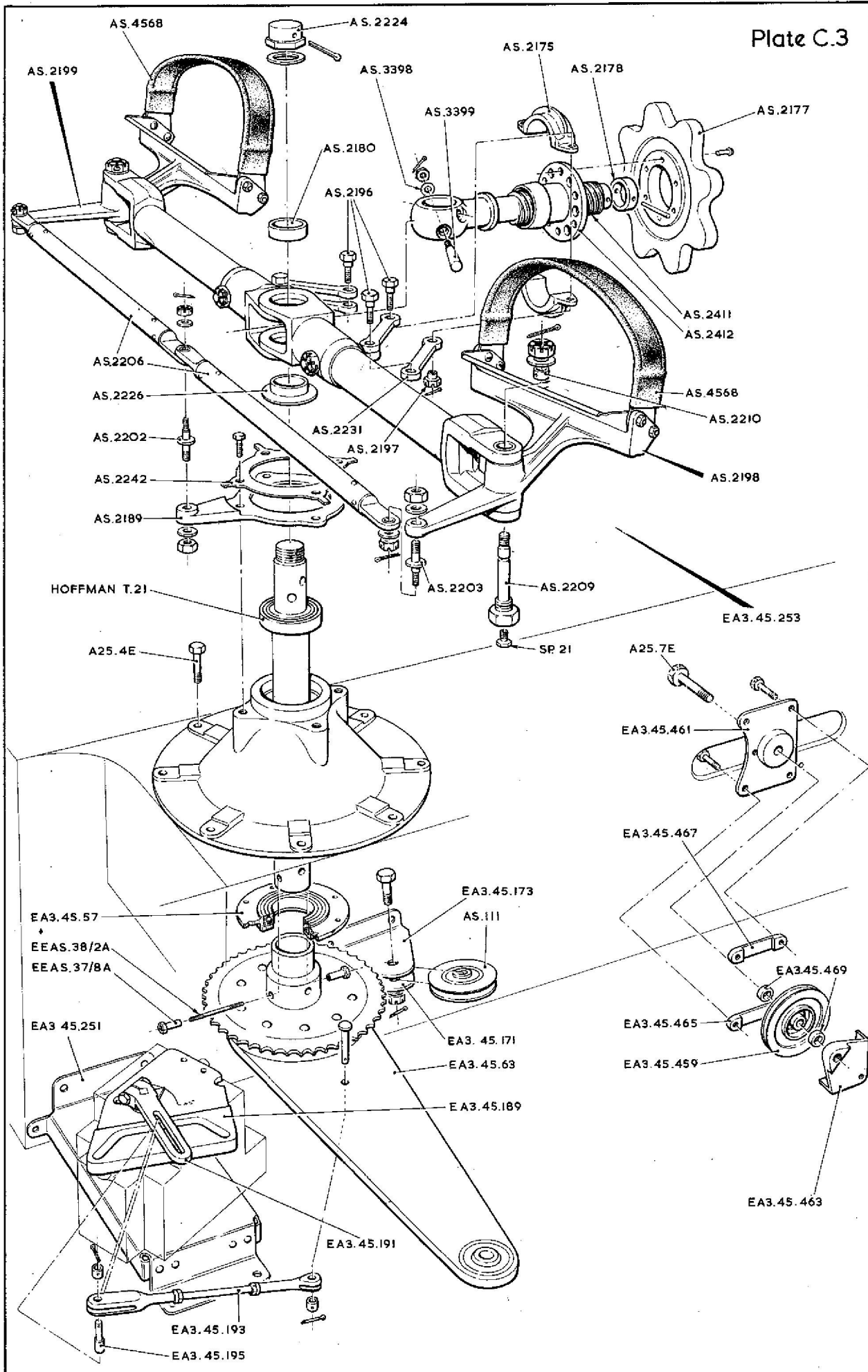
PILOTS RUDDER PEDALS
