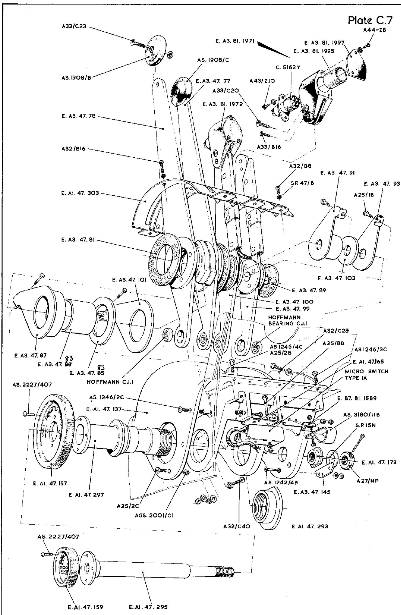
PILOTS THROTTLE BOX
