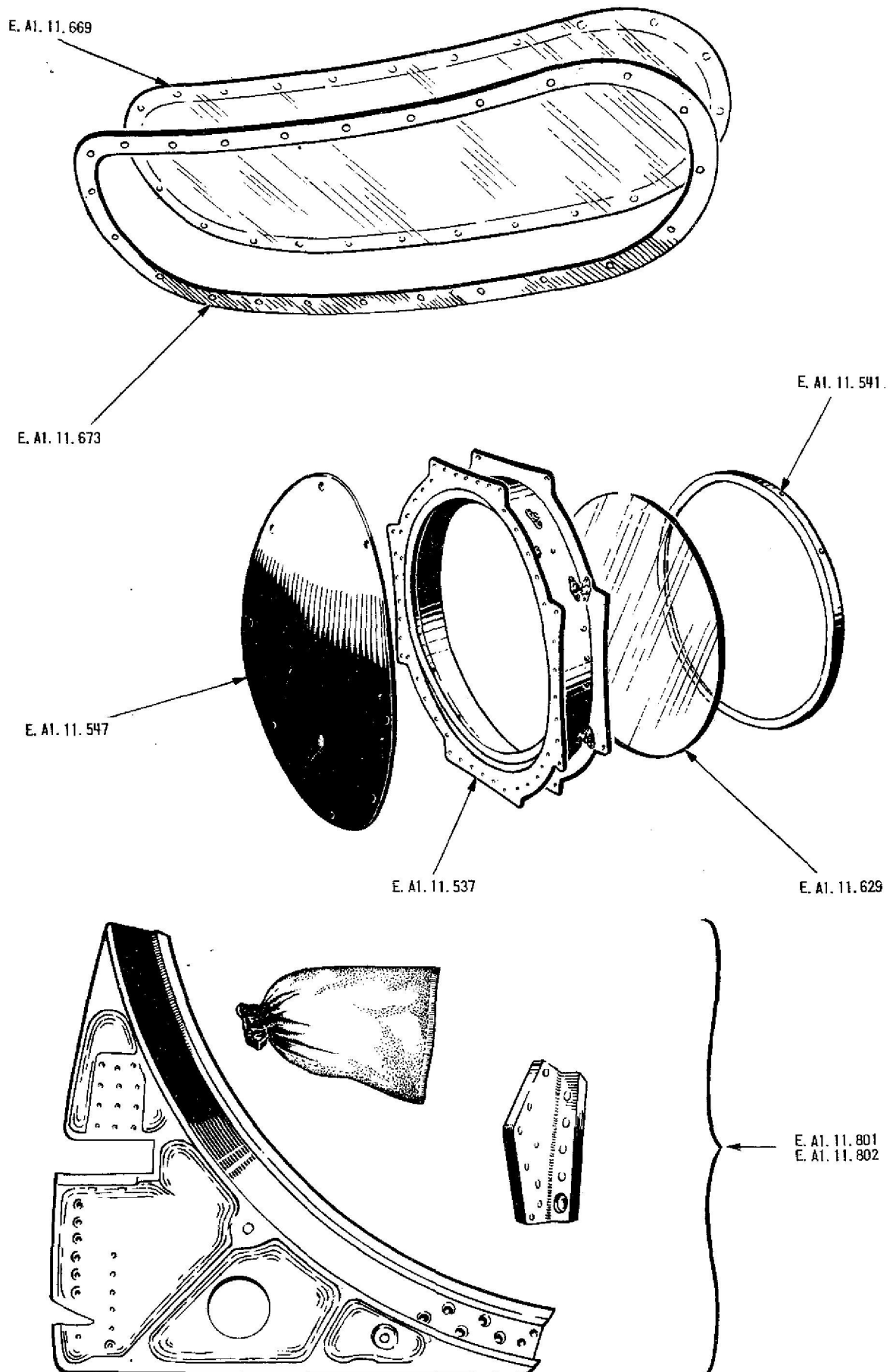
CENTRE FUSELAGE STRUCTURE EQUIPMENT
