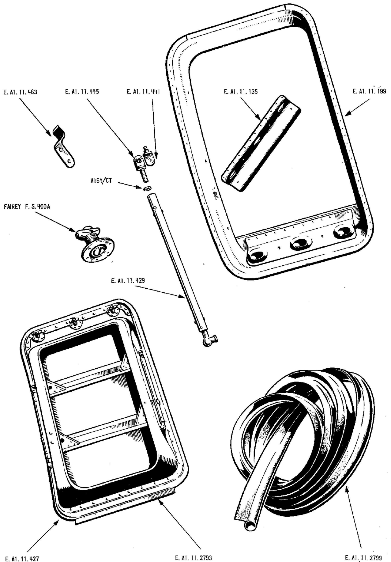
CENTRE FUSELAGE STRUCTURE - ACCUMULATOR DOOR AND FRAME
