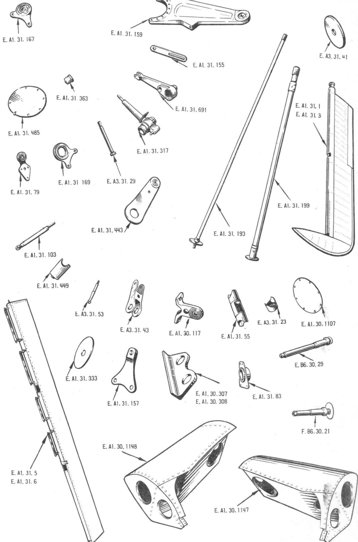
TAILPLANE AND ELEVATORS
