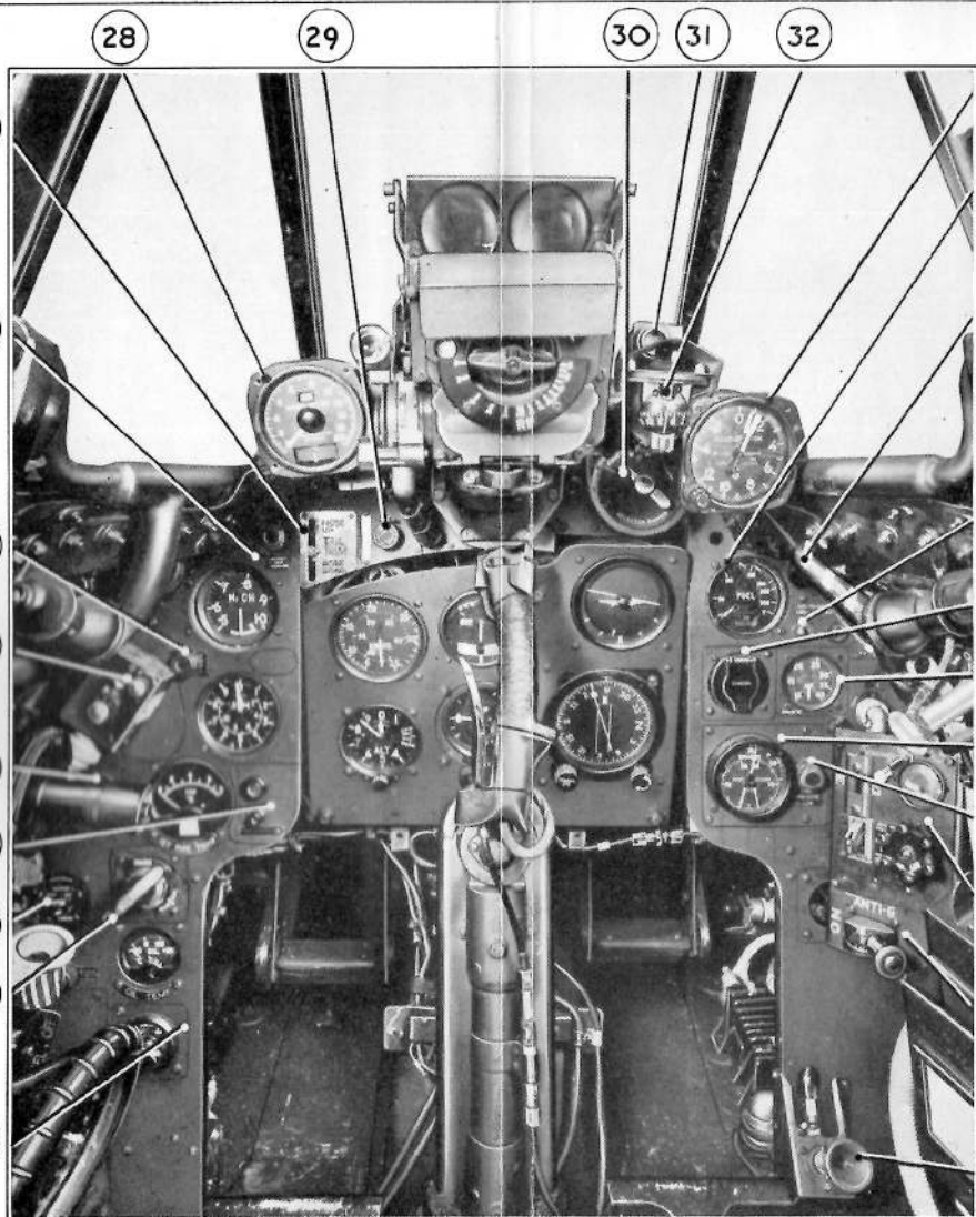
FIG 2 COCKPIT — FORWARD VIEW
