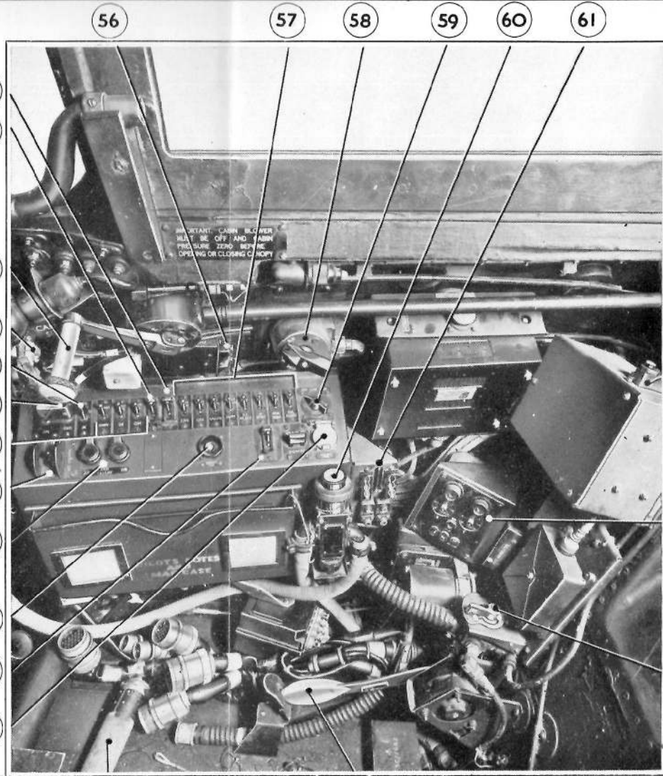
FIG 3 COCKPIT — STARBOARD SIDE
