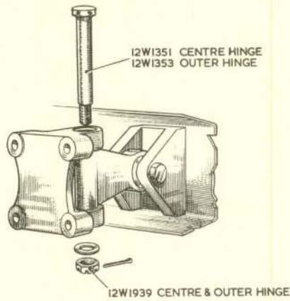
AILERON ATTACHING PARTS
