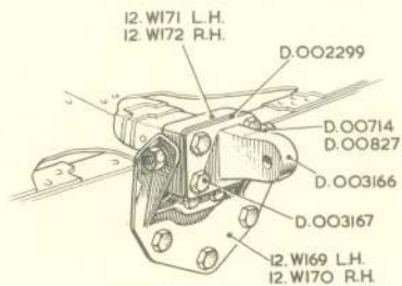
WING JOINT 'C'
