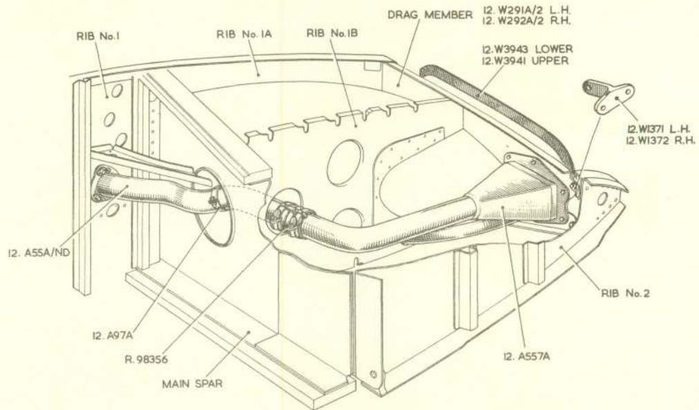
STARBOARD WING
