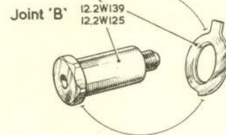
JOINTS 'A' & 'B', MAINPLANE TO FUSELAGE
