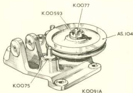
Detail 'D' BRACKET PORT, AILERON PULLEY & TORQUE LEVER.
