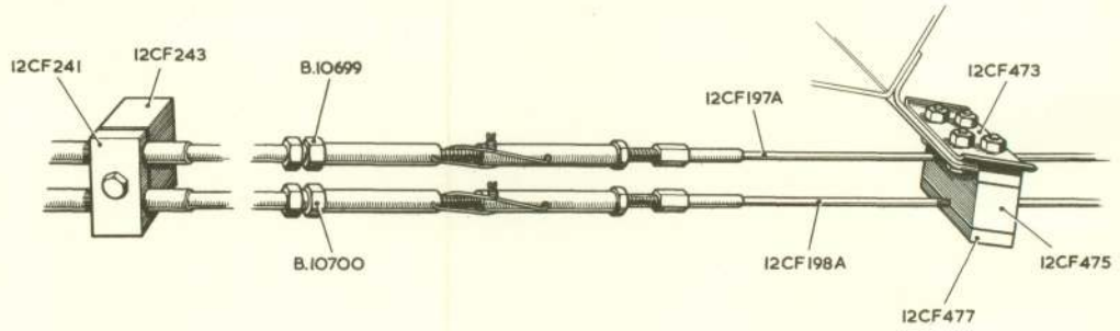
ELEVATOR TRIM CONTROL RUN ON FALSE SPAR.
