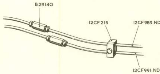
ELEVATOR TRIM CONTROL RUN ON FALSE SPAR.
