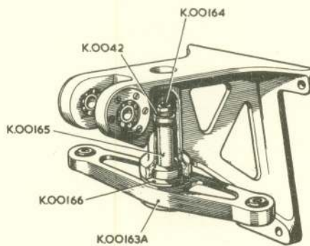
K.OO171A BRACKET. CENTRE SUPPORT.
