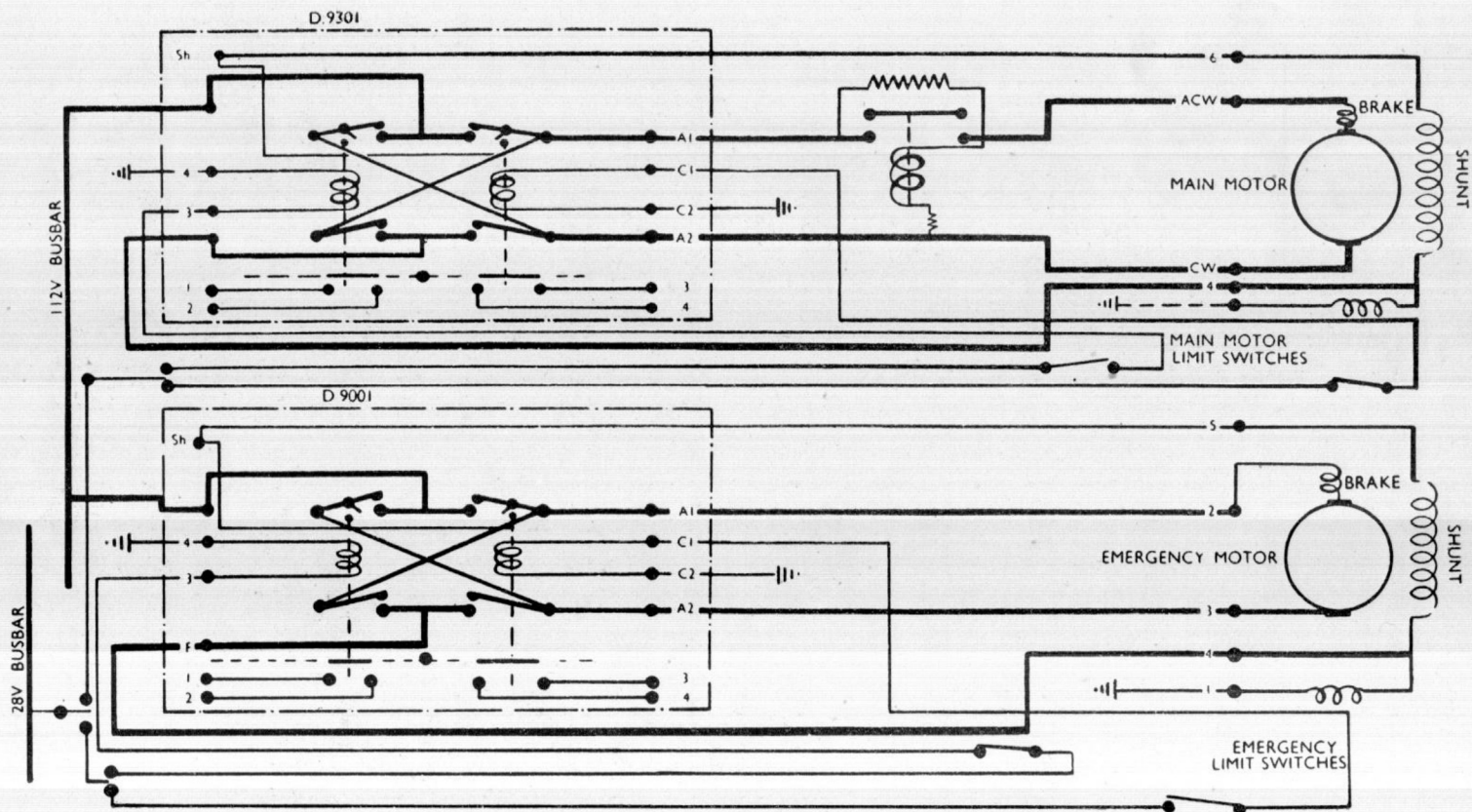
Fig. 4. Typical installation wiring diagram
