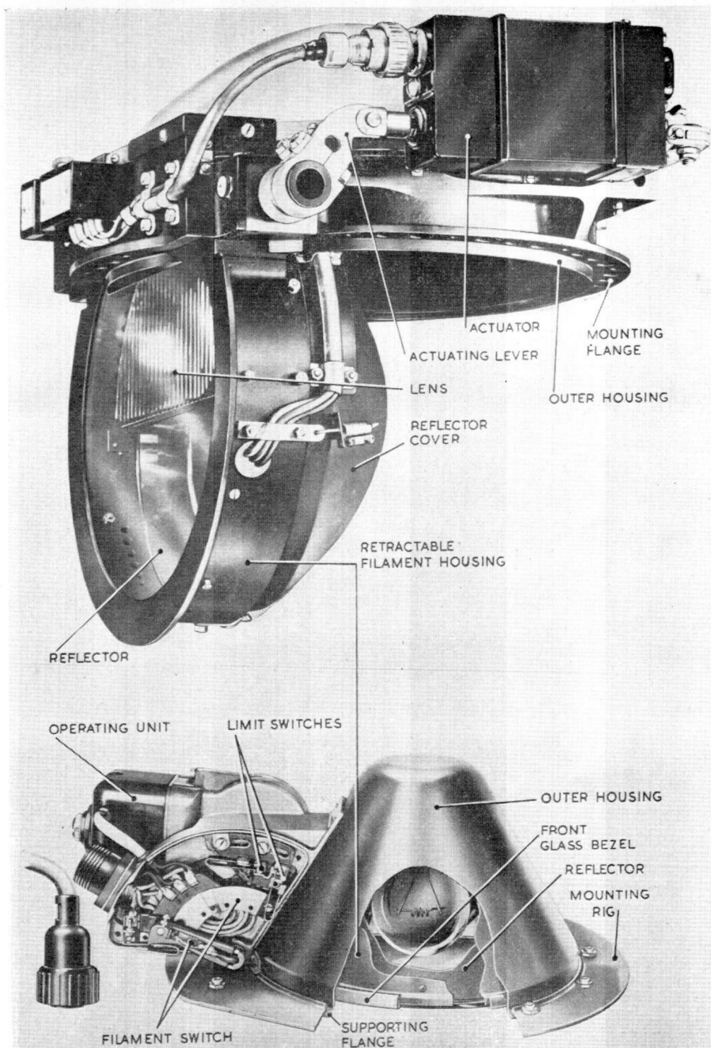
Fig. 2. Typical lamp assemblies
