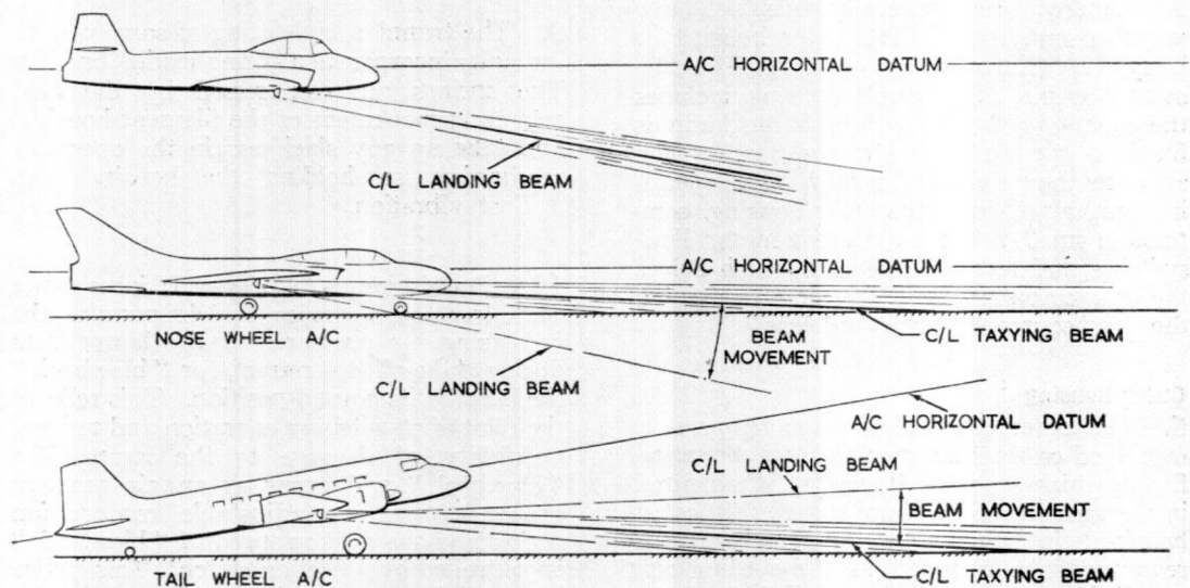
Fig. 1. Beam movement with attitude change
