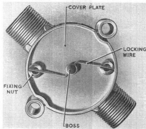
Fig. 3 Cover plate
