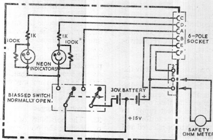
Fig. 9. Circuit diagram of detector test kit
