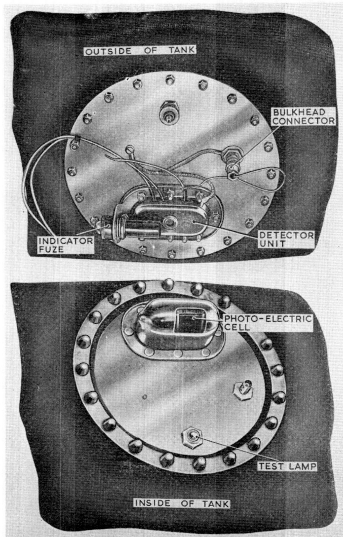
Fig. 2. Detector unit installed on tank access panel
