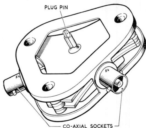
Fig. 6. Terminal block
