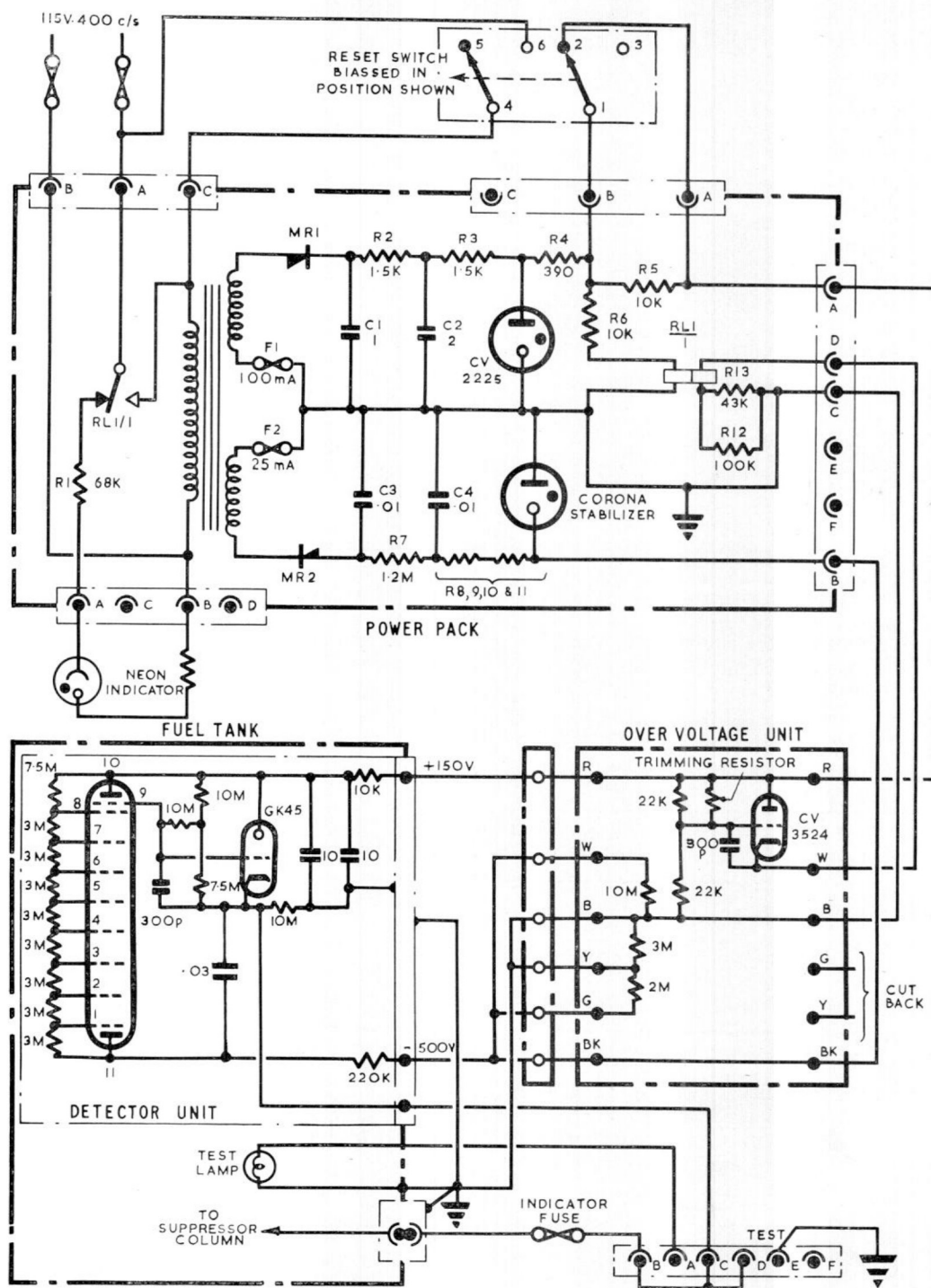
Fig. 8. Circuit diagram of typical installation
