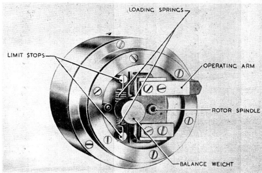
Fig. 13. Hunter, operating arm details
