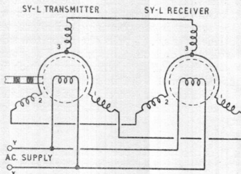
Fig. 9. Circuit diagram, synchronous link
