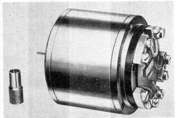
Fig. 3. Magslip receiver
