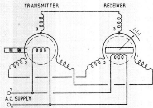
Fig. 7. Circuit diagram for single receiver
