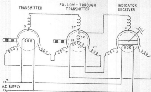
Fig. 8. Circuit diagram for differential indication
