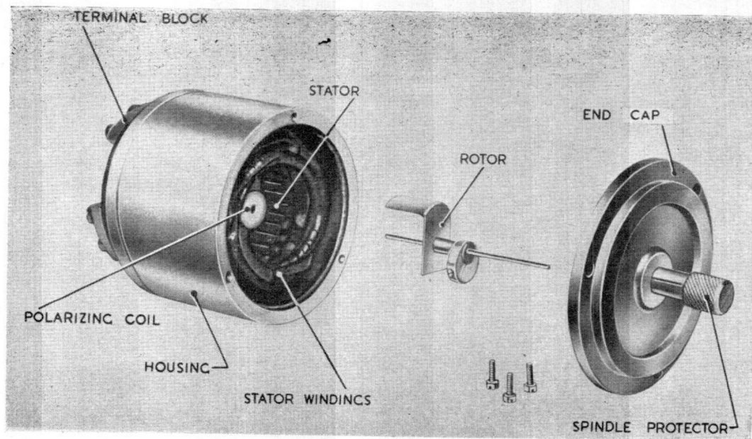
Fig. 4. Receiver partly dismantled
