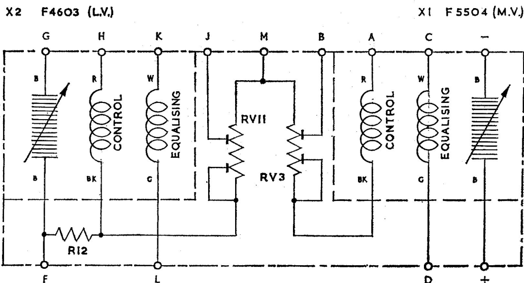
Fig. 3. Circuit diagram
