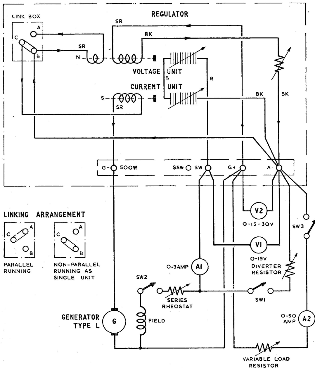
Fig. 1. Test circuit diagram
