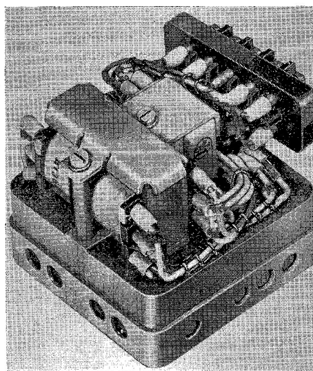
Fig. 2. View of unit with cover removed
