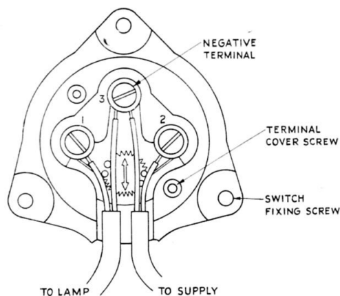
Fig. 4. Terminals with cables connected
