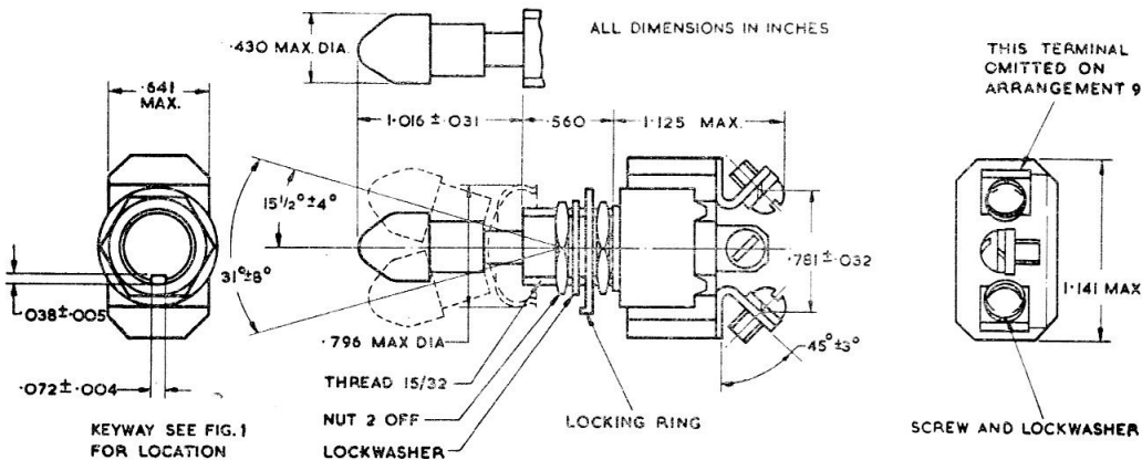
Fig. 2. Installation details
