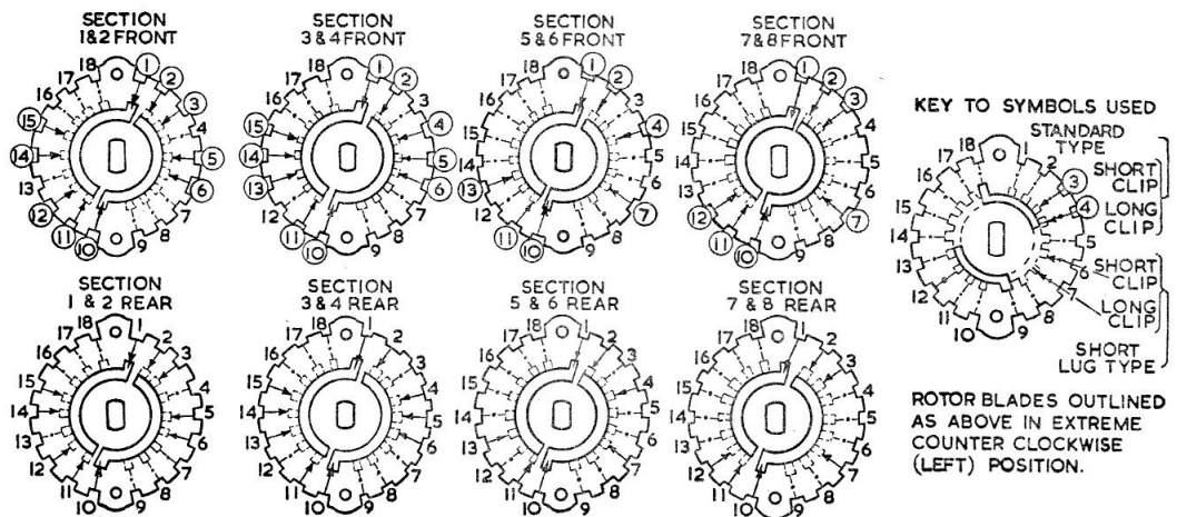
Fig. 1. Switch section contact arrangements
