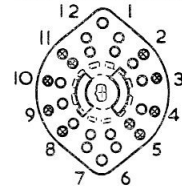
Fig. 1. Switch section contact arrangements
