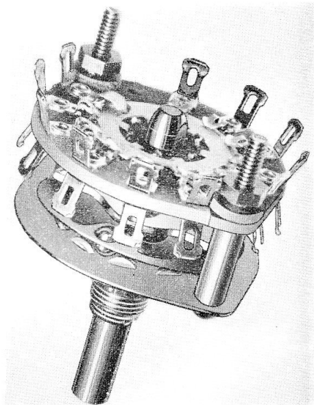
Fig. 2. Switch mechanism
