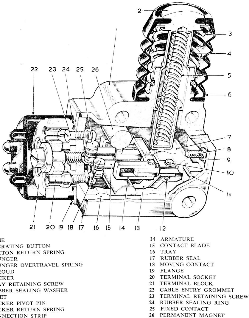
Fig. 2. Sectional view of microswitch
