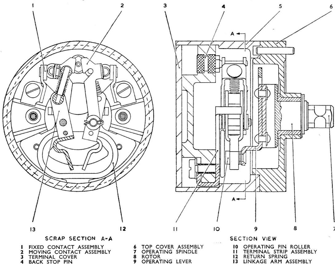
Fig. 1. Sectioned view of Type 2B, No. 2 switch
