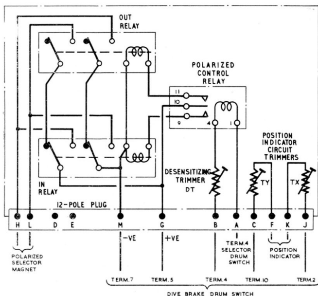
Fig. 2. Circuit diagram
