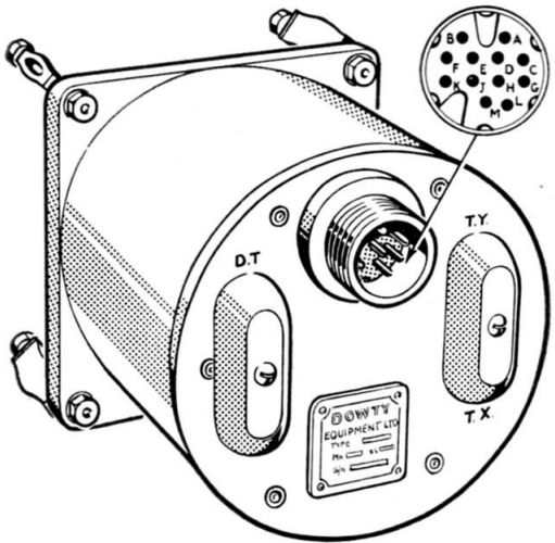
Fig. 1. Single relay panel unit, Type C5101Y, Mk. 2
