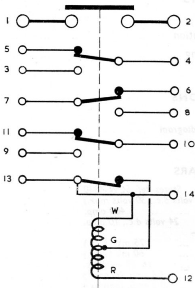
Fig. 2. Circuit diagram
