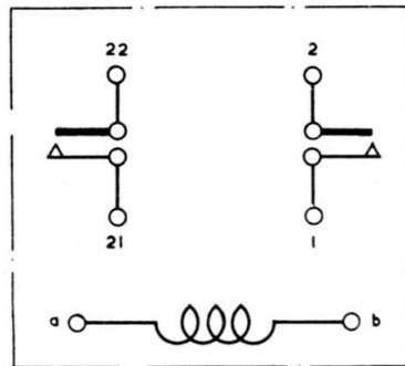
Fig. 2. Circuit diagram
