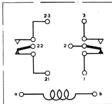
Fig. 2. Circuit diagram
