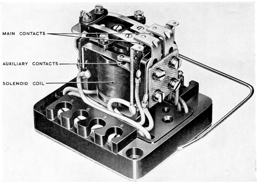
Fig. 1. Type 2A, No. 2 magnetic switch
