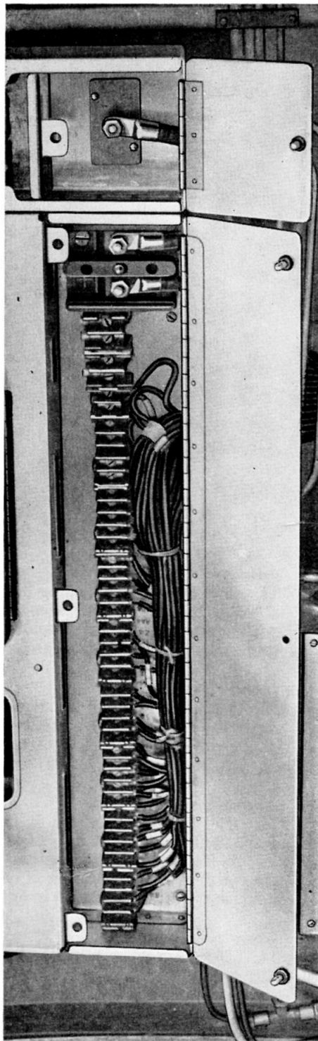
Fig. 6. Typical cable loom, showing cable ends prepared for various terminals
