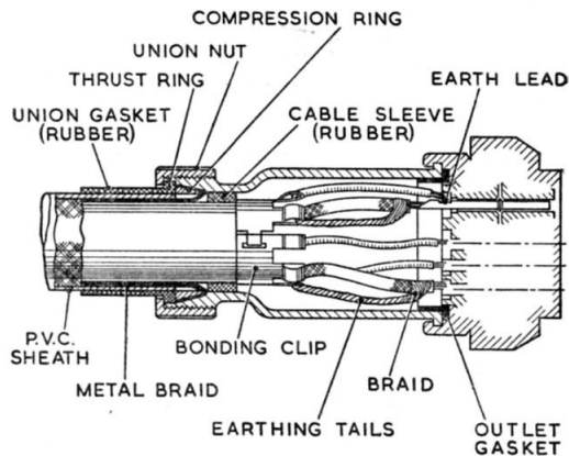
Fig. 12. Method of wiring 2kV cable units
