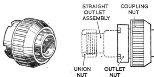
Fig. 1. Typical plug (free)
