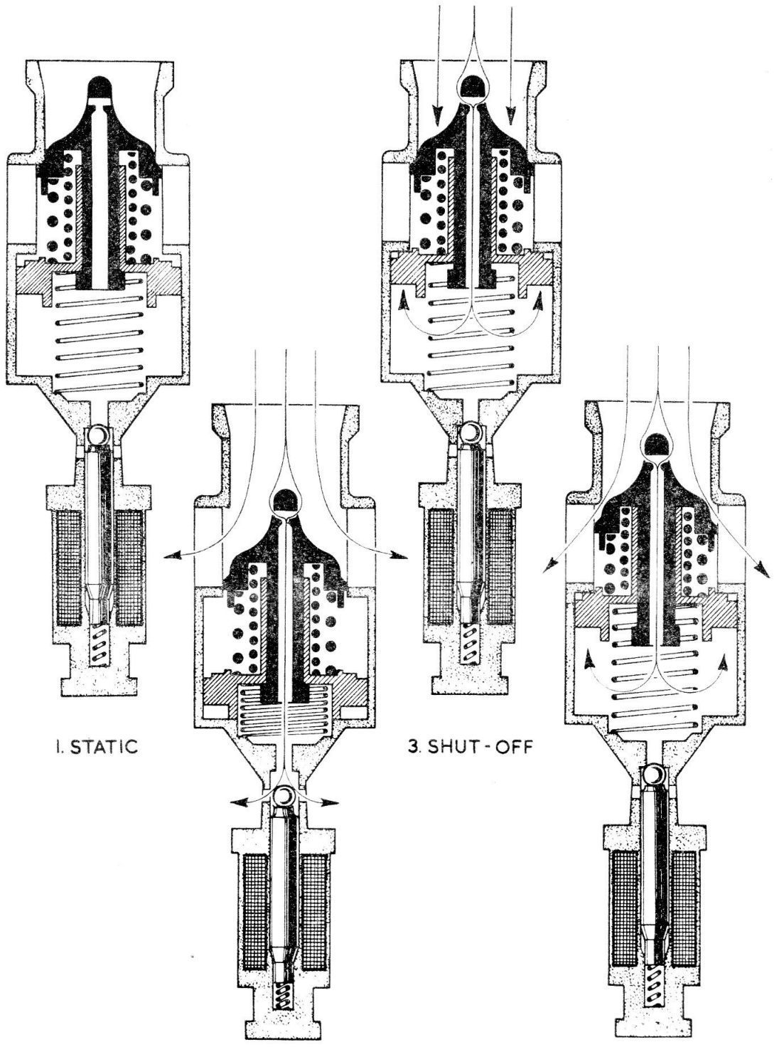
Fig. 4. Functional diagram
