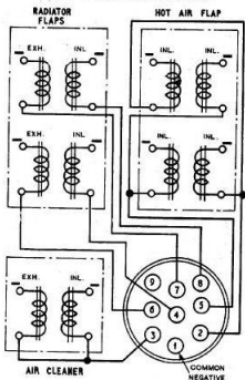
Fig. 7. Diagram of connections for electromatic valve (AC1031)
