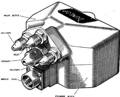
Fig. 1. Duo-electric valve (AC1130)
