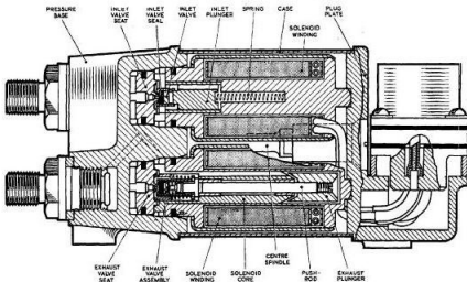
Fig. 5. Sectional view of electromagnetic valve (AC1119)
