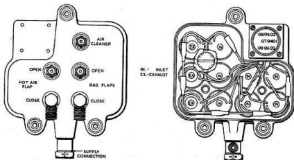
Fig. 6. Electromatic valve (AC1031)
