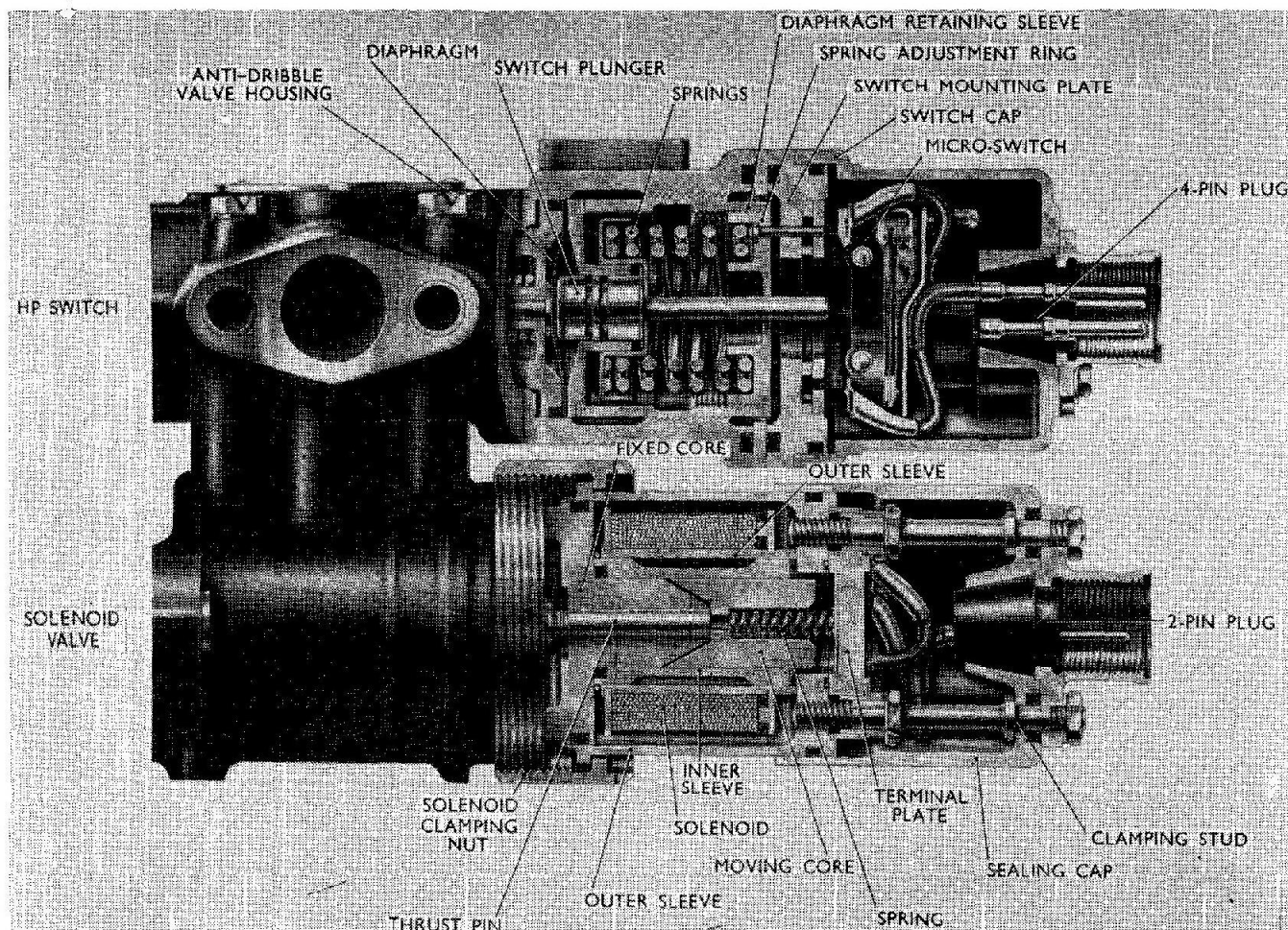
Fig. 1 Sectional view of high pressure switch and solenoid valve
