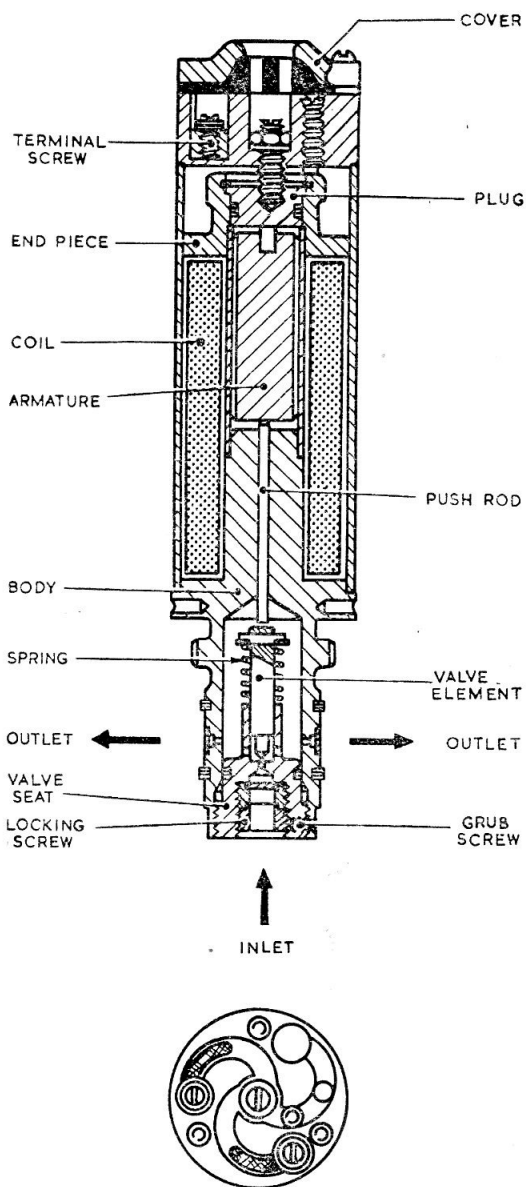
VIEW WITH COVER REMOVED Fig. 3. Electro-hydraulic valve, Type AI403
