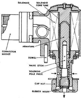
Fig. 2. General arrangement of valve
