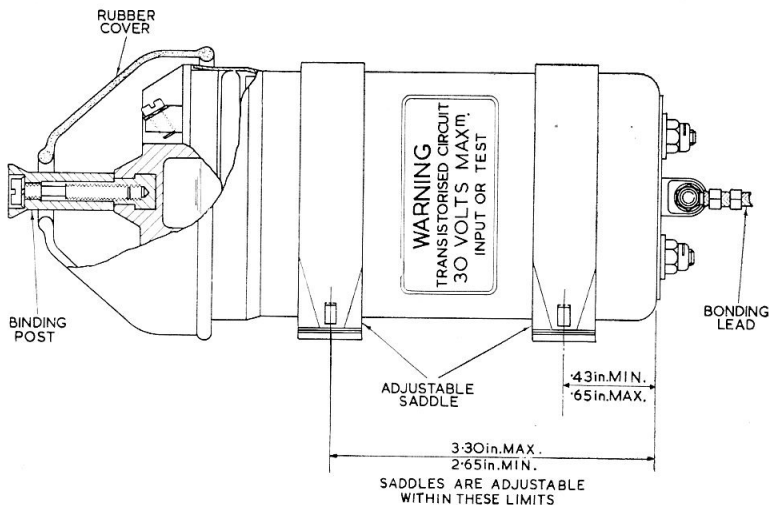
Fig. 1. Part section view of typical control unit
