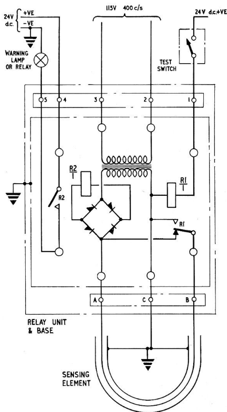
Fig. 3. Circuit diagram
