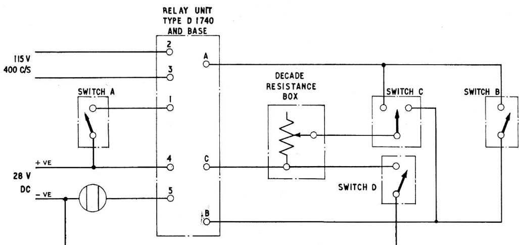
Fig. 1. Test circuit diagram
