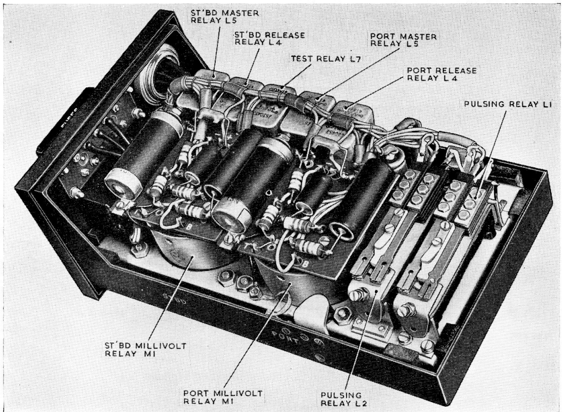
Fig. 2. Control unit with cover removed
