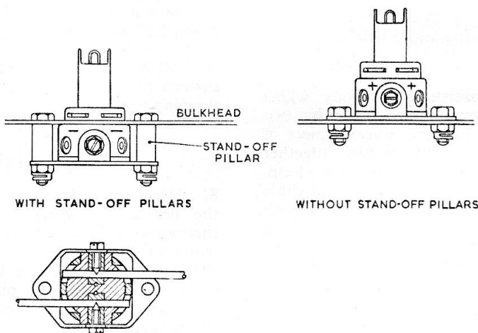
Fig. 2. Installation with and without Stand-off pillars
