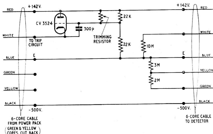
Fig. 2. Circuit diagram
