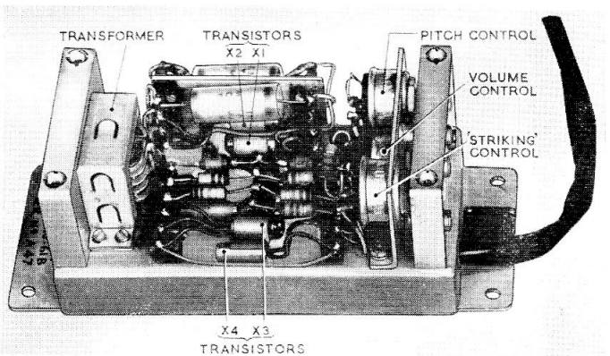
Fig. 1. View of unit from above (cover removed)
