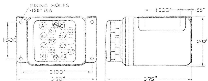
Fig. 6. Installation diagram
