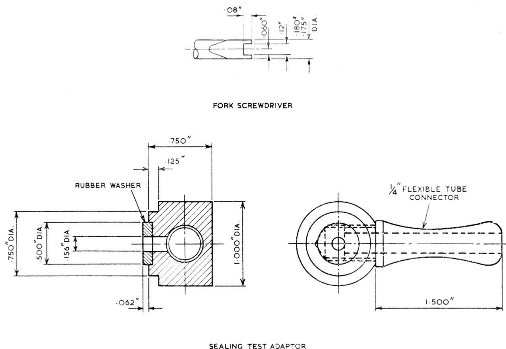
Fig. 5. Special tools
