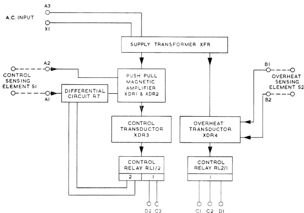
Fig. 3. Block schematic diagram
