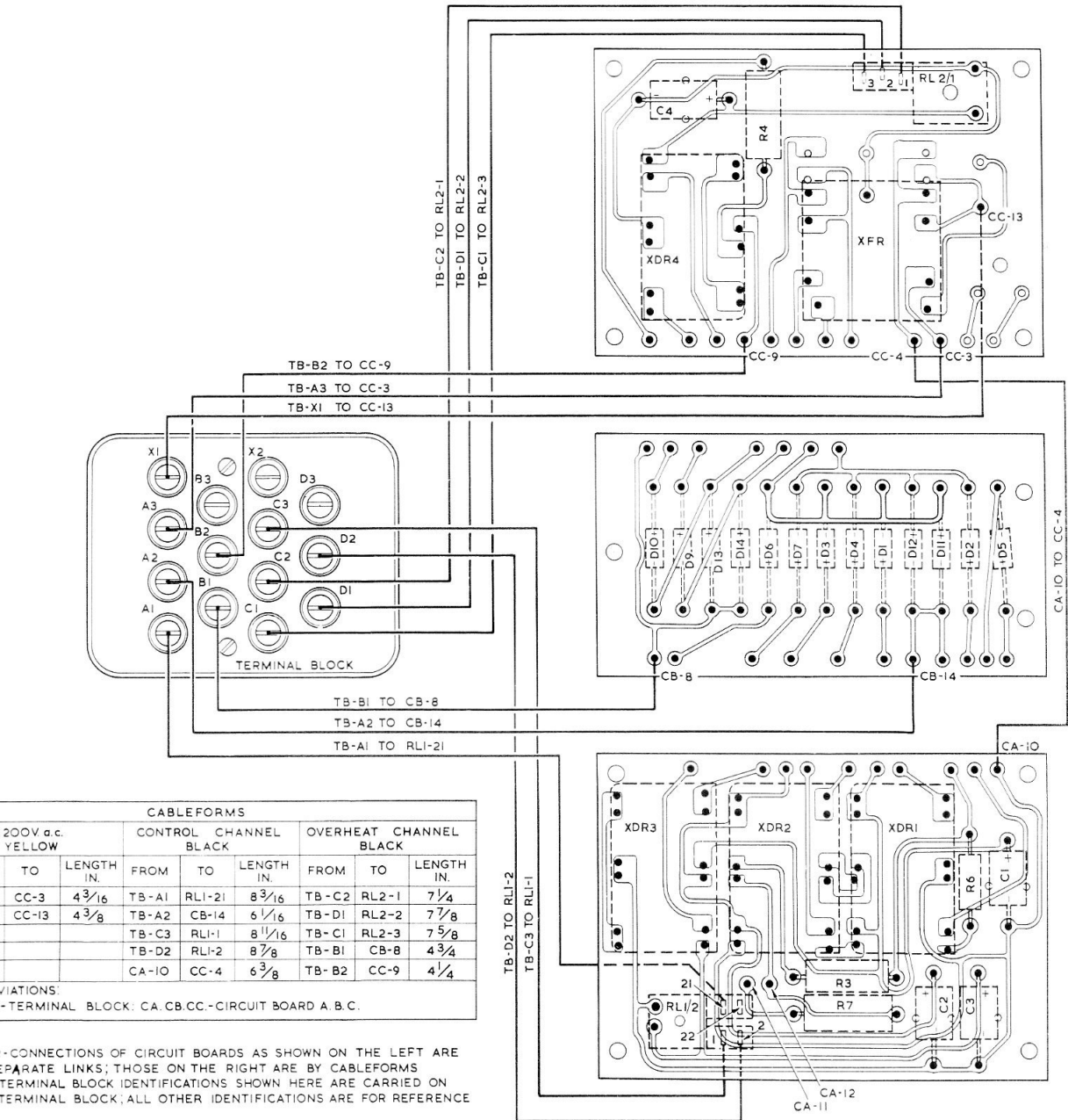
Component layout and wiring diagram RESTRICTED
