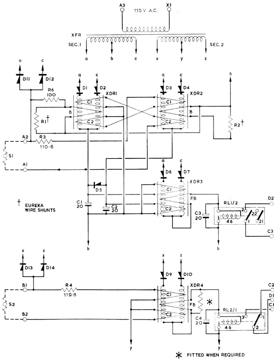
Fig. 4. Circuit diagram
