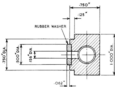
SEALING TEST ADAPTOR
