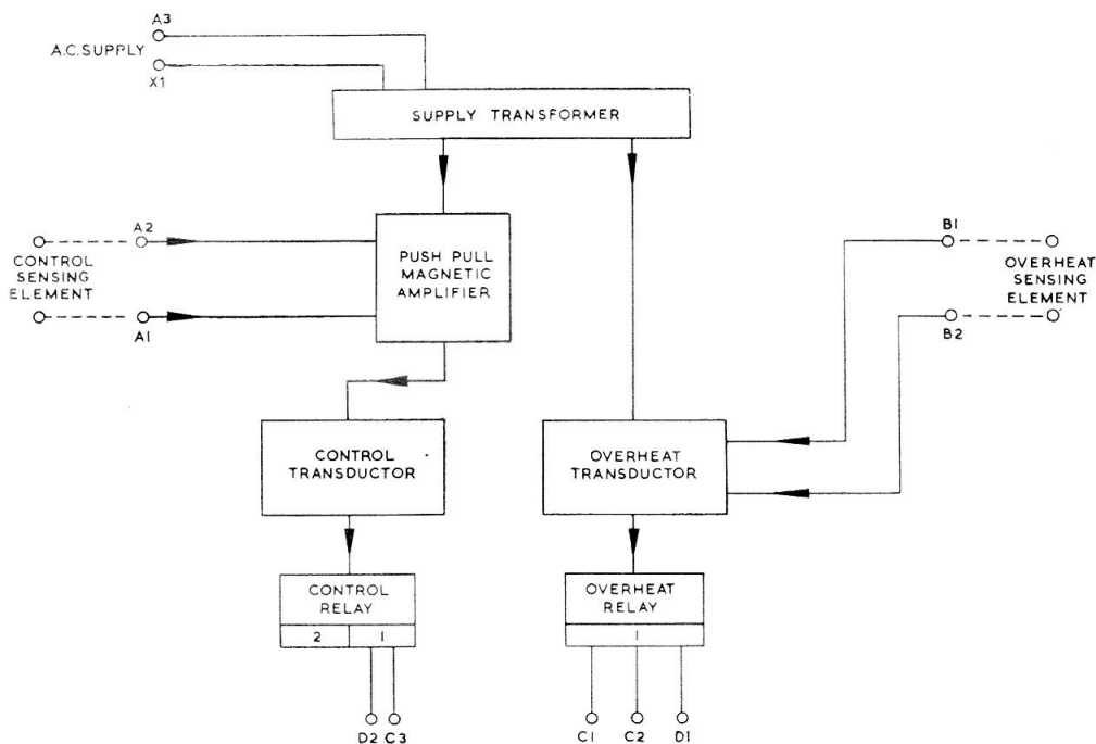
Fig. 3. Block diagram
