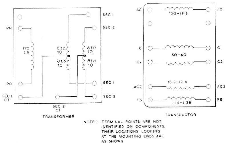
Fig. 6. Transformer and transducer winding resistances
