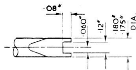
FORK SCREWDRIVER
