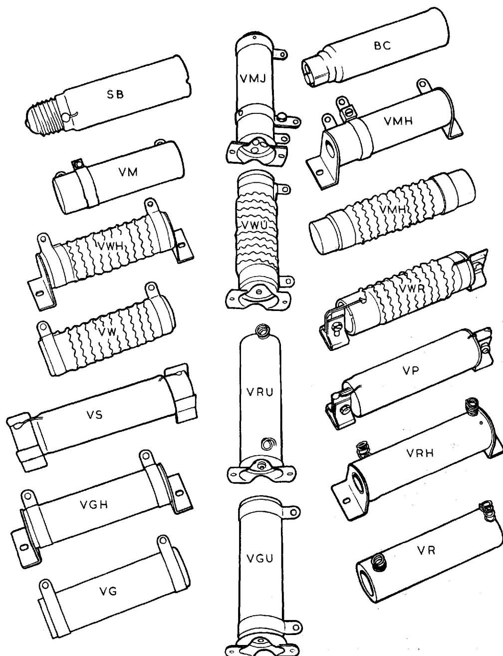
Fig. 2. 'K' type tubular resistors and mountings
