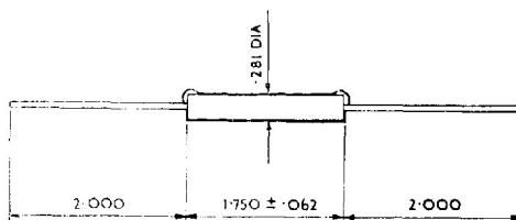
Fig 1. Resistor, Rotax, Type N79776
