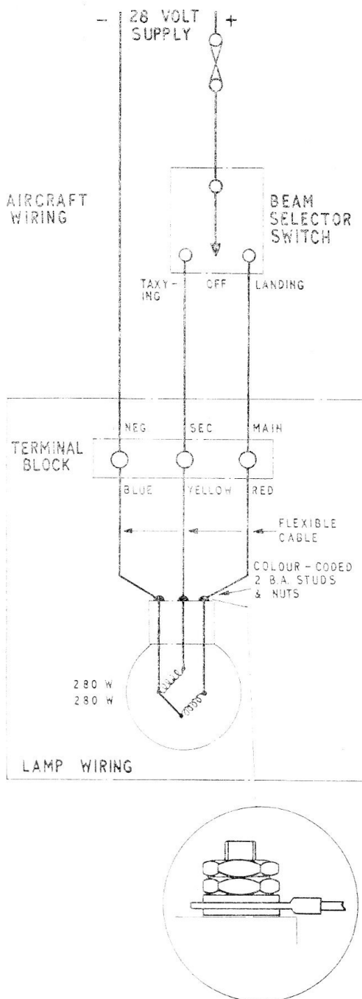
Fig. 2. Circuit diagram
