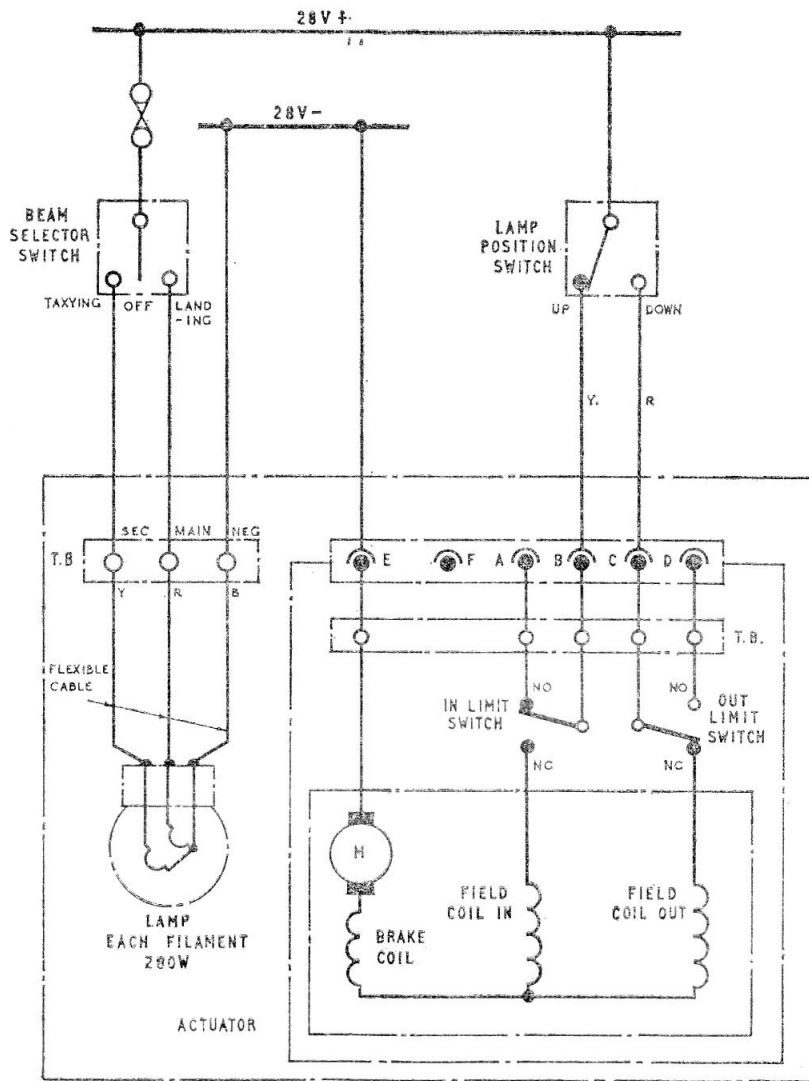
Fig. 2. Circuit Diagram
