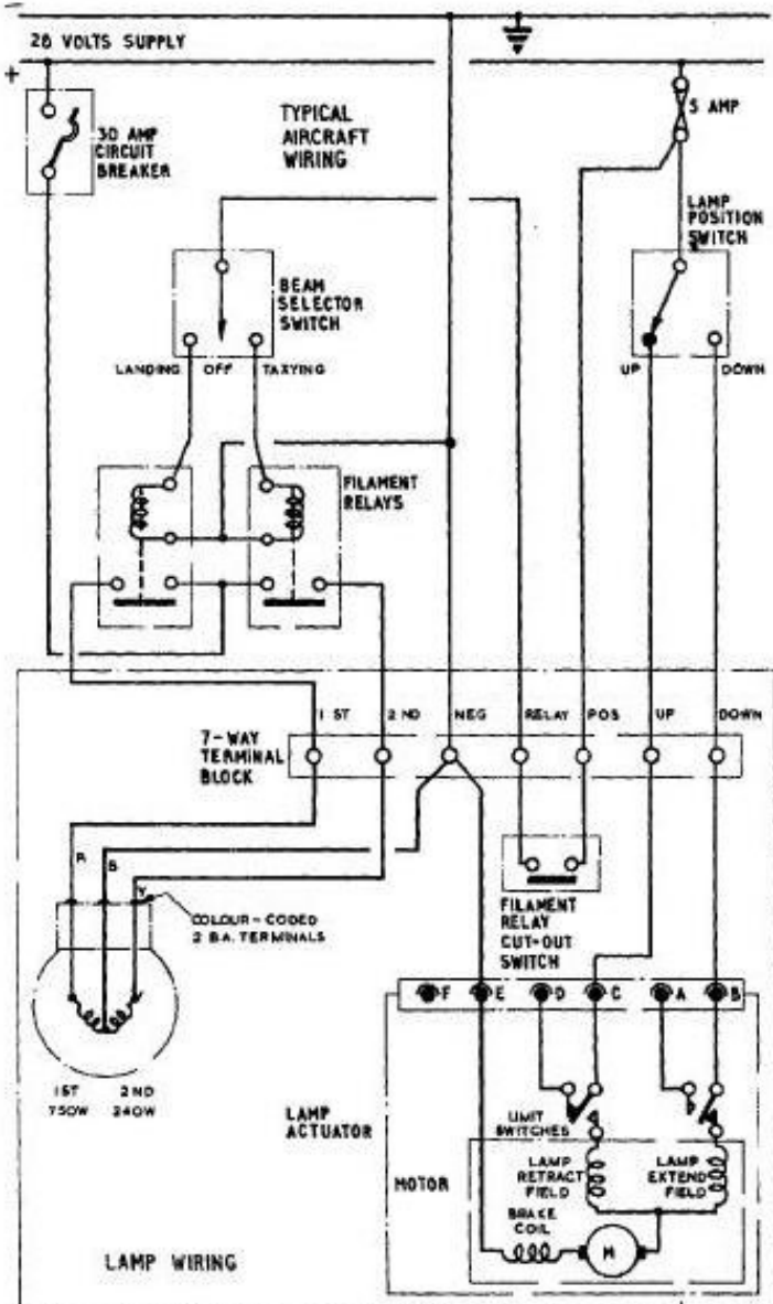
Fig. 2. Circuit diagram
