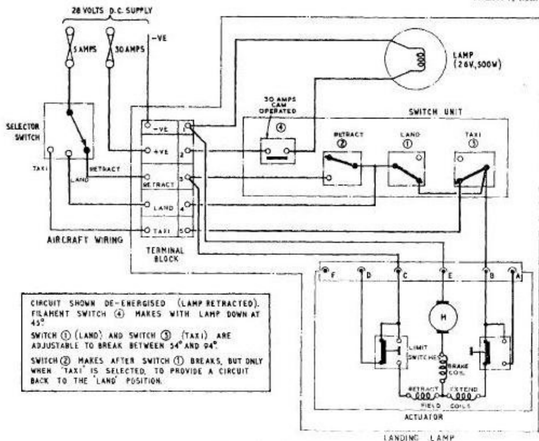
Fig. 4. Circuit diagram
